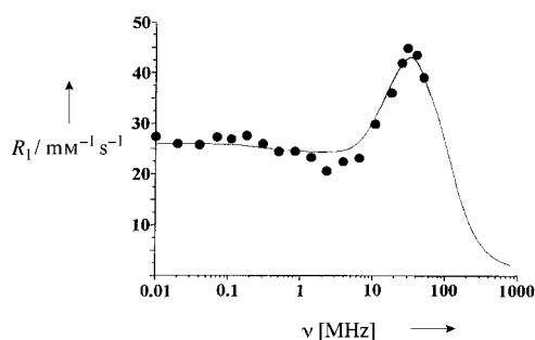
Figure 3. NMRD profile of the [\text{Gd}^{\text{III}}(\mathbf{1})] -HSA adduct 25 °C. The best-fit curve was calculated with the parameters: \Delta = 0.023 \text{ cm}^{-1} , \tau_R = 1.75 \text{ ns} , \tau_V = 12 \text{ ps} , D(\text{ZFS}) = 0.24 \text{ cm}^{-1} , \tau_M = 38 \text{ ns} , q = 1 , r = 3.1 \text{ \AA} ; \nu = proton Larmor frequency, R_1 = longitudinal water-proton relaxivity, \tau_V = correlation time for electron relaxation, D(\text{ZFS}) = static zero-field splitting.
